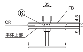
“c”部詳細 (2箇所)
