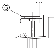
“b”部詳細 (4箇所)
